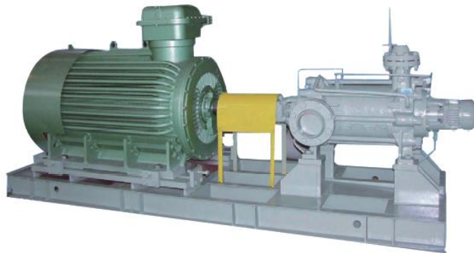
DS 卧式高压多级泵 High Pressure Stage Casing Pumps API 610 BB4 Type
